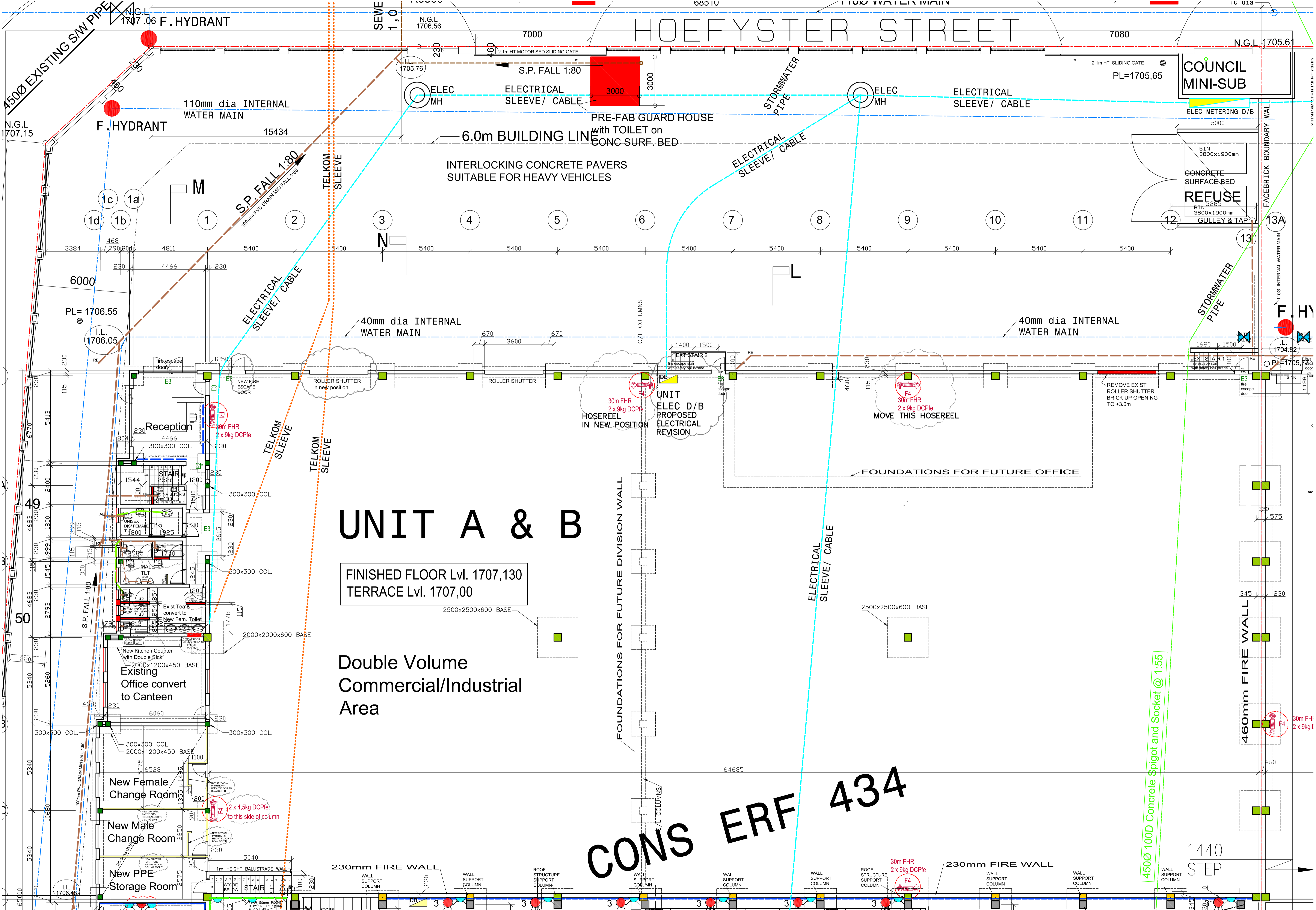
STORMMILL X 5: UNITS A & B- tenant BAOBAB LAYOUT PLAN DATED 25 APRIL 2018
